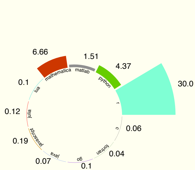
fib
