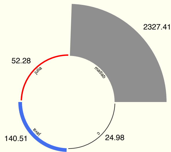
printfd
