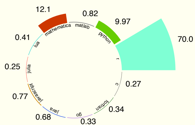
recursion_quicksort
