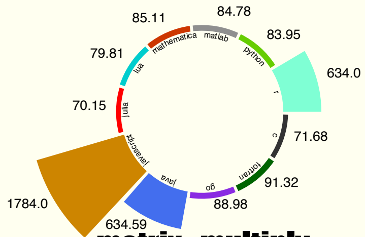
matrix_multiply
