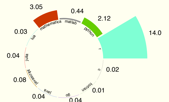
recursion_fibonacci
