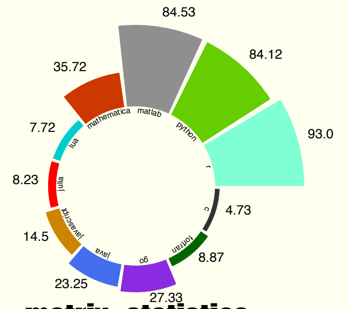
matrix_statistics
