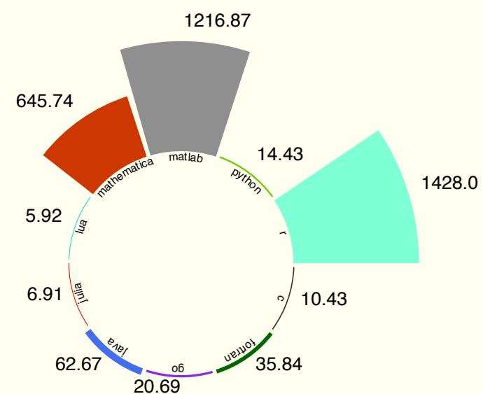
print_to_file
